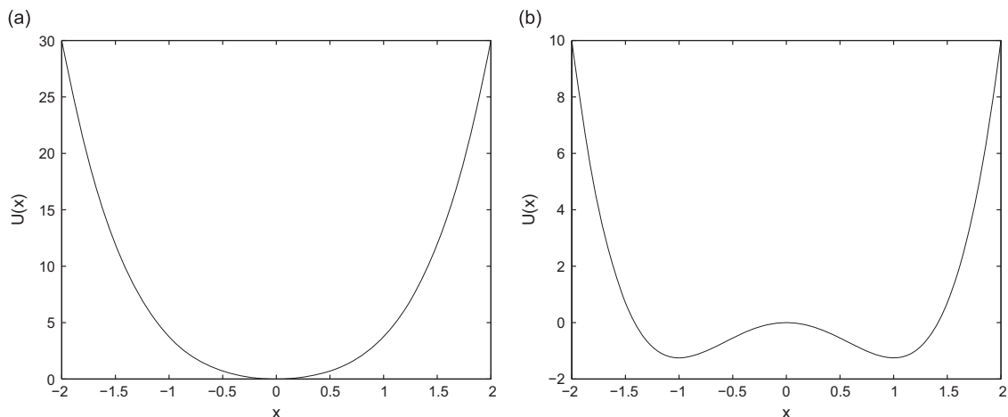
Fig. 2. The shapes of potential function U(x) = \frac{1}{2}\hat{k}_1 x^2 + \frac{1}{4}\hat{k}_3 x^4 . (a) The monostable potential function with \hat{k}_1 > 0 and \hat{k}_3 > 0 . (b) The bistable potential function with \hat{k}_1 < 0 and \hat{k}_3 > 0 .
